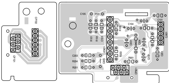
(Relay board)
