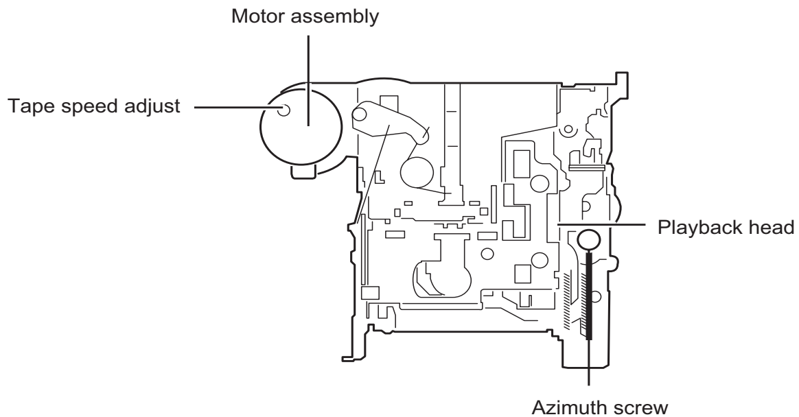
Cassette mechanism (Surface)
